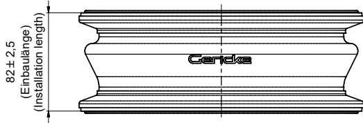
DN 200
