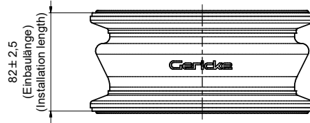
DN 150
