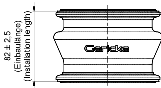
DN 100
