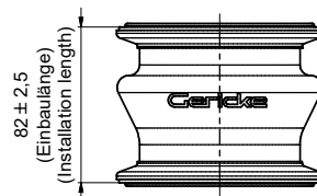
DN 80
